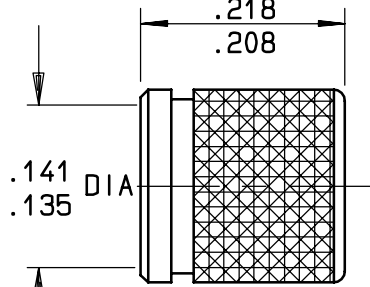
INNER FERRULE
