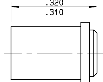
DIELECTRIC SLEEVE
